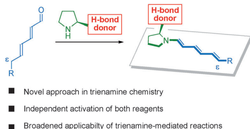
Scheme 1. Remote functionalizations through H-bond-directed trienamine chemistry.
